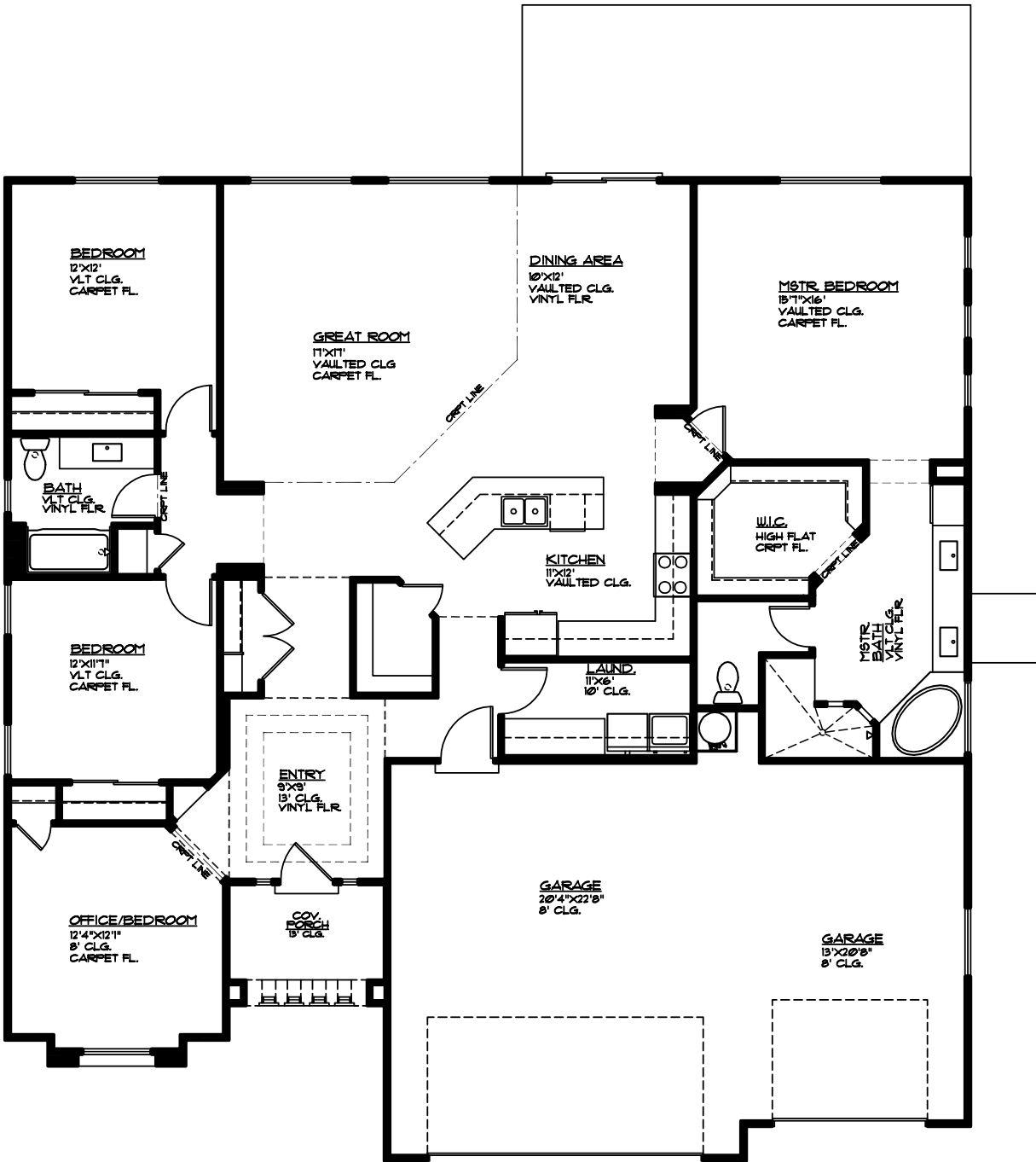
MAIN FLOOR PLAN MAIN FLOOR = 2165 SQ. FT. GARAGE AREA = 765 SQ. FT.
