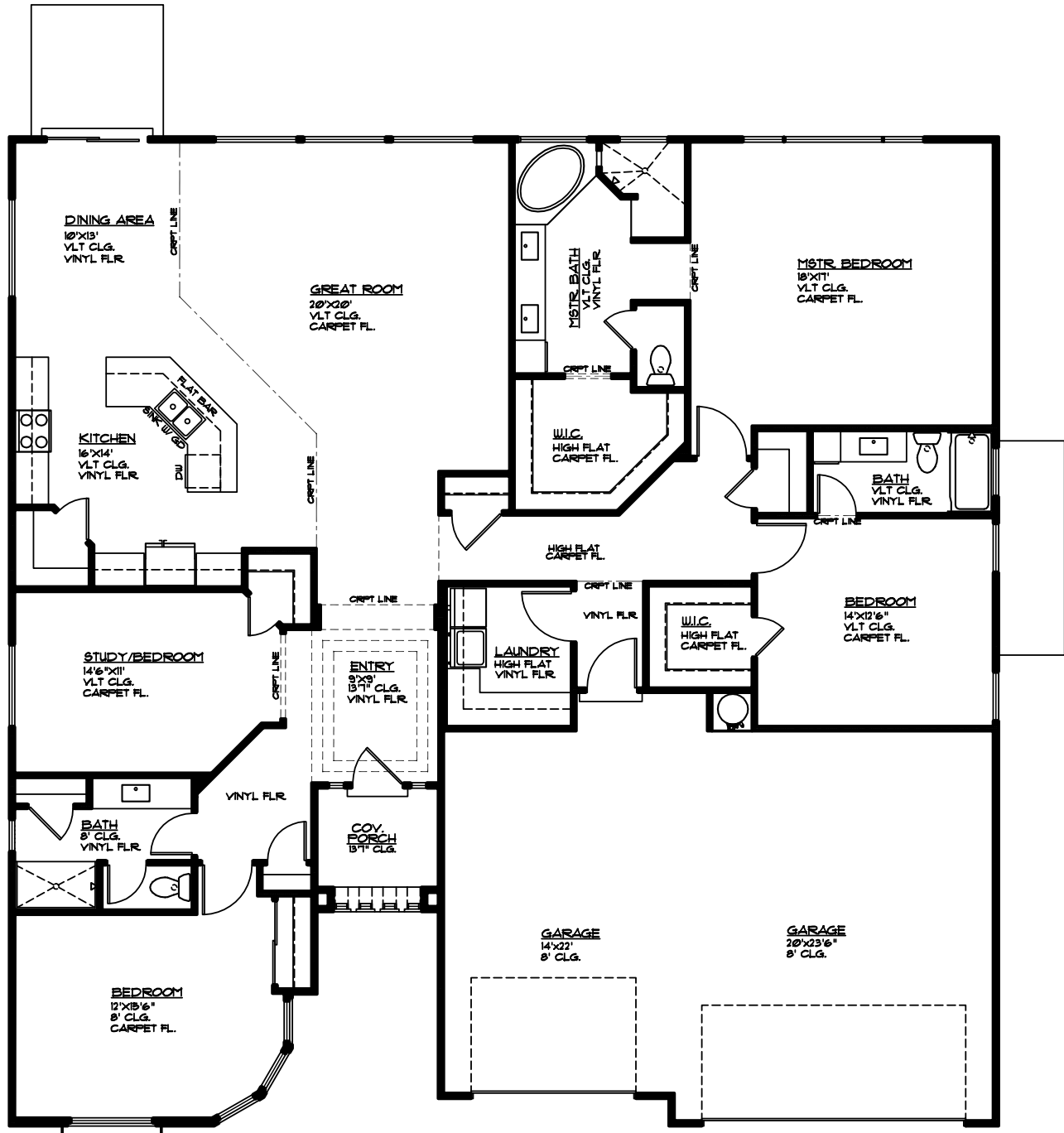
MAIN FLOOR PLAN MAIN FLOOR = 2586 SQ. FT. GARAGE AREA = 811 SQ. FT. COV. PORCH = 55 SQ. FT.
