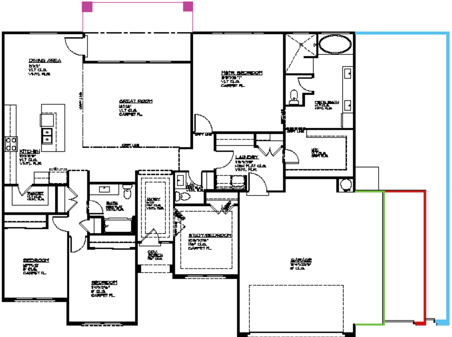
MAIN FLOOR PLAN MAIN FLOOR 2218 SQ. FT.
