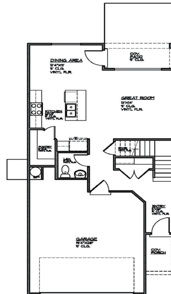
MAIN FLOOR PLAN MAIN FLOOR - 698 SQ. FT. GARAGE AREA - 440 SQ. FT. COV. PORCH - 40 SQ. FT. COV. PATIO - 60 SQ. FT.
