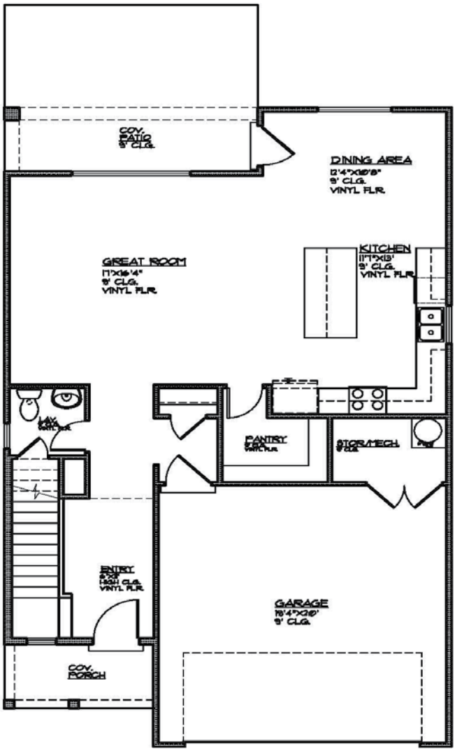
MAIN FLOOR PLAN MAIN FLOOR - 880 SQ. FT. GARAGE AREA - 450 SQ. FT. COV. PORCH - 55 SQ. FT. COV. PATIO - 55 SQ. FT.
