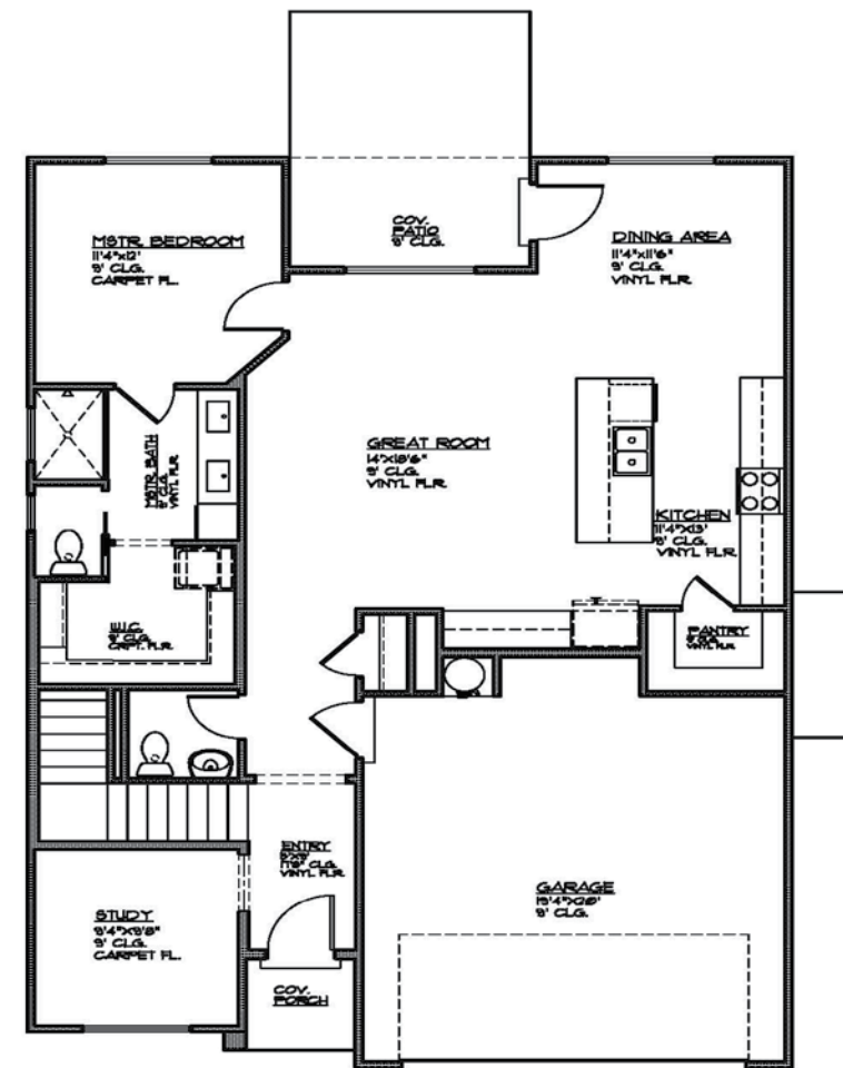
MAIN FLOOR PLAN MAIN FLOOR - 1210 SQ. FT. GARAGE AREA - 425 SQ. FT. COV. PORCH - 25 SQ. FT. COV. PATIO - 66 SQ. FT.
