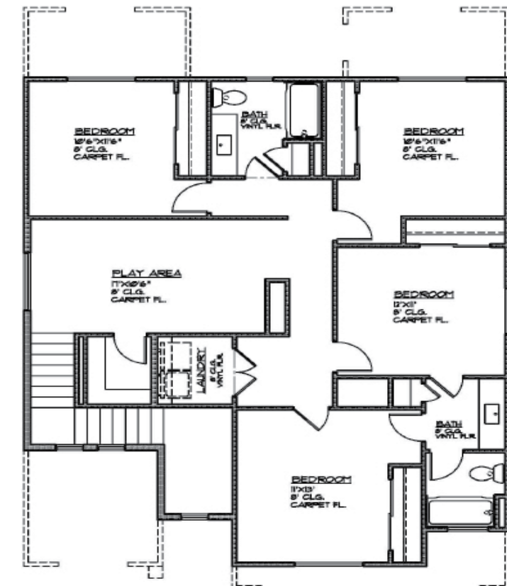
UPPER FLOOR PLAN UPPER FLOOR - 1234 SQ. FT.
