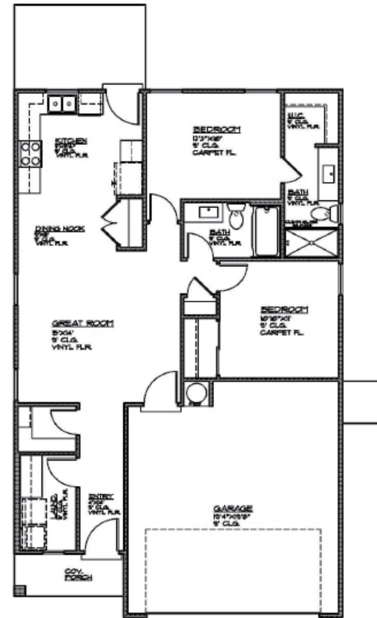
MAIN FLOOR PLAN MAIN FLOOR - 1010 SQ. FT. GARAGE AREA - 430 SQ. FT. COV. PORCH - 40 SQ. FT.
