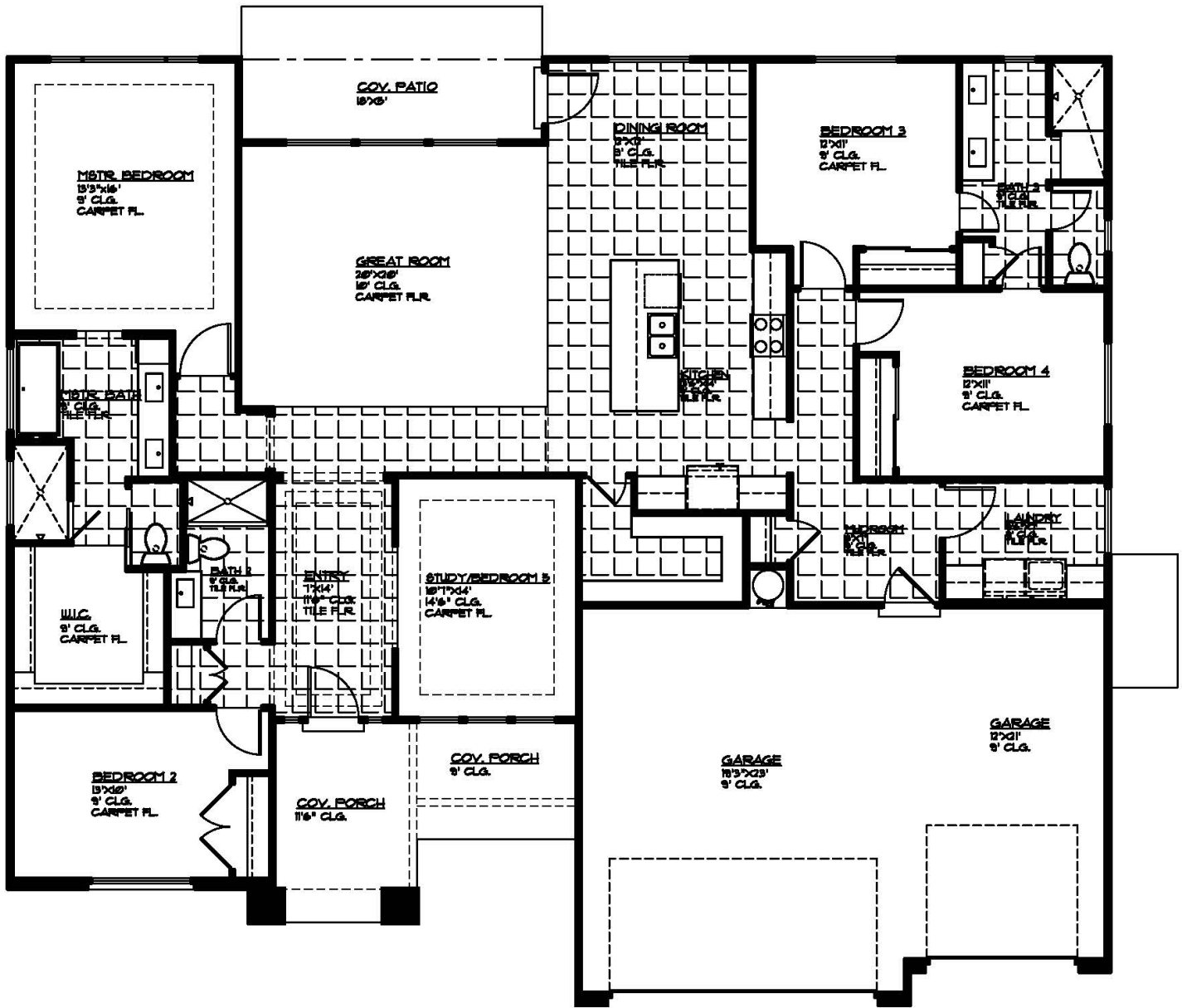
MAIN FLOOR PLAN MAIN FLOOR - 2472 SQ. FT. GARAGE AREA - 158 SQ. FT. COV. PORCH - 168 SQ. FT. COV. PATIO - 90 SQ. FT.
